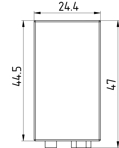
Battery Front
